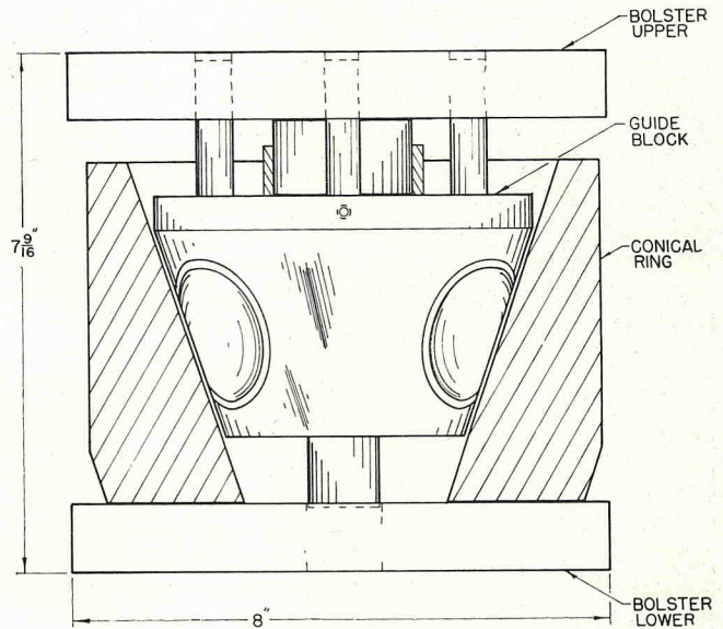
FIGURE 4. Sectional drawing of wedge-type apparatus showing guide block inside conical ring.
